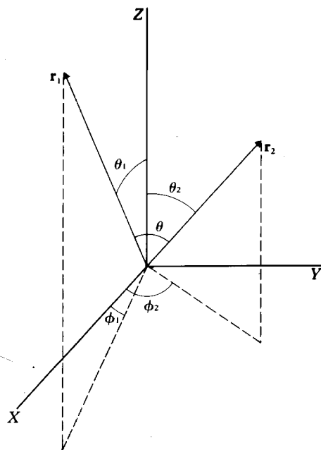
6.7 The polar coordinates of vectors r_1 and r_2 .
